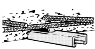
Continuous Concrete Insert PS 349 1 3/8" x 1 3/8" x 12 ga. 3'-20' lengths
